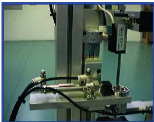
Fig. 4. Measuring manipulator
