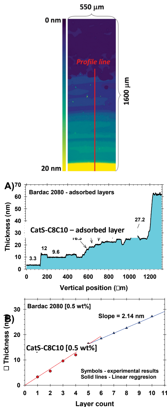
Fig. 4. Experimental results of 0.5% CatS-C8C10. A) Images obtained using imaging ellipsometry; B) Thickness of the adsorbed layer at the red profile line shown in A; C) arrangement of the sequence of thickness taken from the profile by their value.
