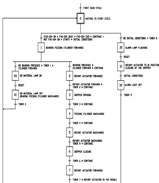
Fig. 8. Program for the feeding module.
