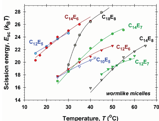
Fig. 3. Dependence of the scission energy of C_n E_m micelles on temperature. Solid lines show the theoretical predictions.
