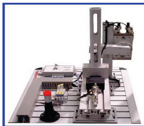
Fig. 3. Manipulators of the feeding module.
