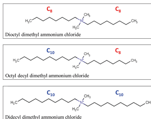
Fig. 1. Structural formulas of the used cationic surfactants.
